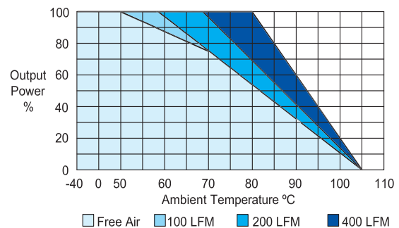
Derating Curve
